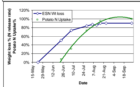
Figure 3. Estimated N release in a Manitoba potato field compared to the typical rate of N uptake by potatoes.
