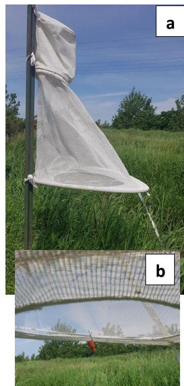
Figure 1. Heliothis trap with 10 cm clearance above grassy weeds and anchor string pulling trap into cone (a). Lure is clipped onto elastic band at the trap opening (b).
